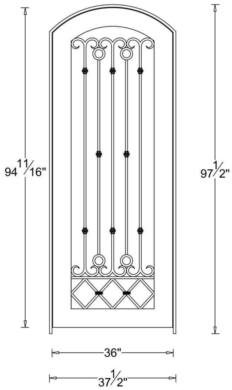
Sequoia 3.0 x 8.0
