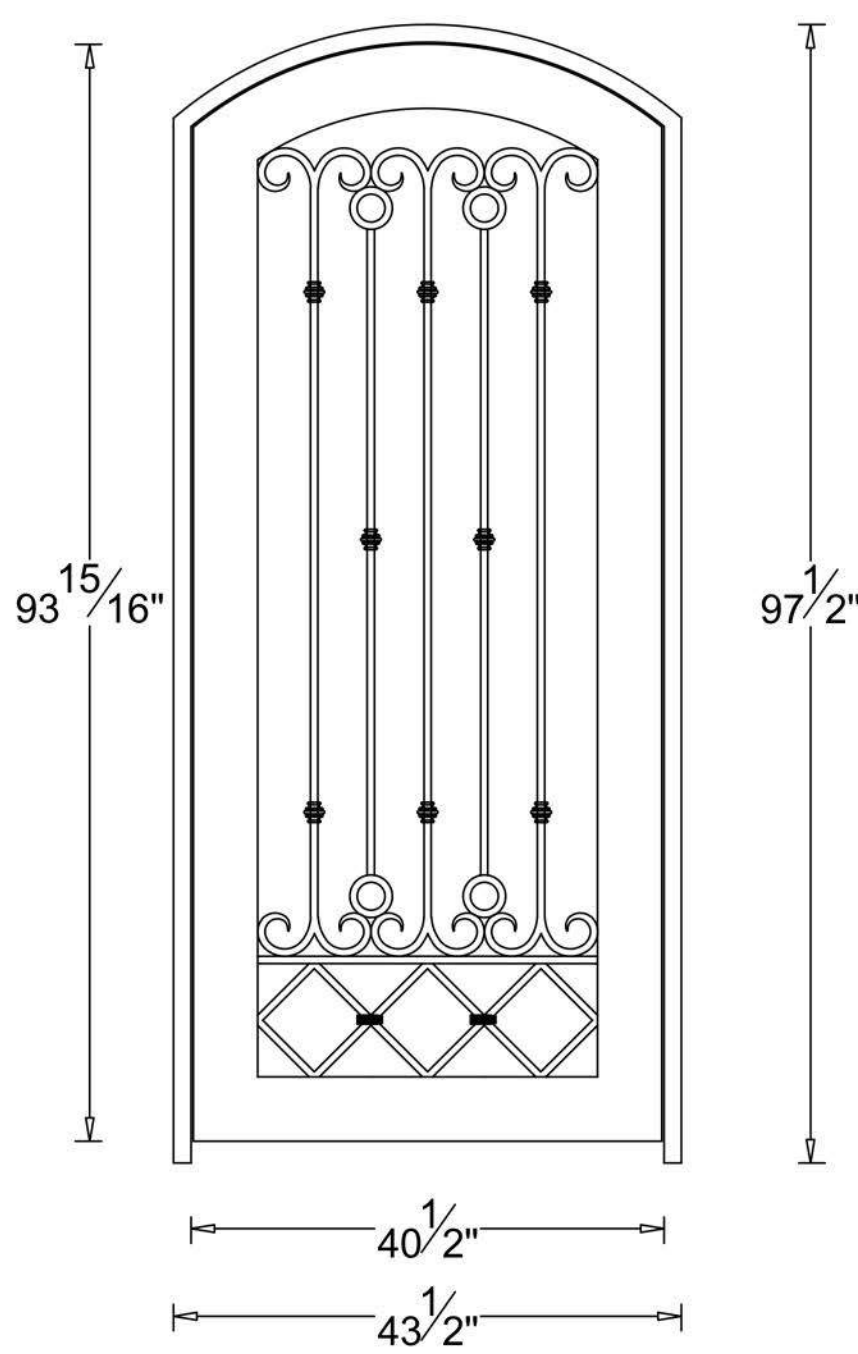
Sequoia 3.6 x 8.0
