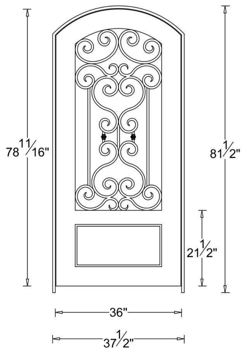
Portland K 3.0 x 6.8
