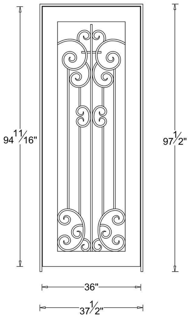
Phoenix 3.0 x 8.0
