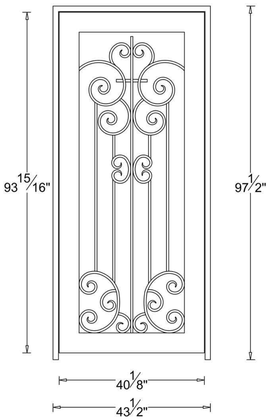
Phoenix 3.6 x 8.0
